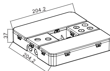
Battery Dimensions
