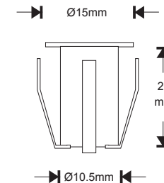
E10PEN-WH Cut out: 11mm
