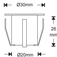
E1030-WH Cut out: 21mm
